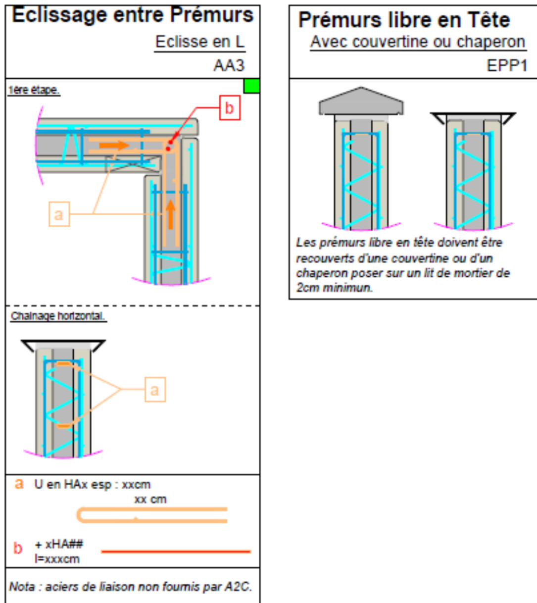
Figure 19 – ACROTÈRES – 2
