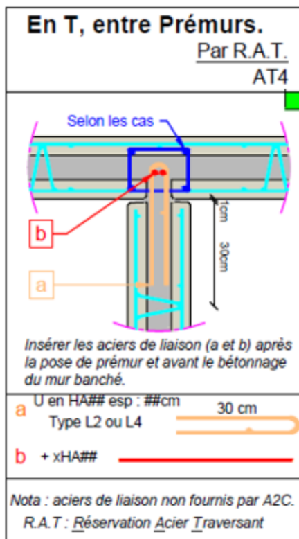
Figure 8 - LIAISONS ARTICULEES – 2
