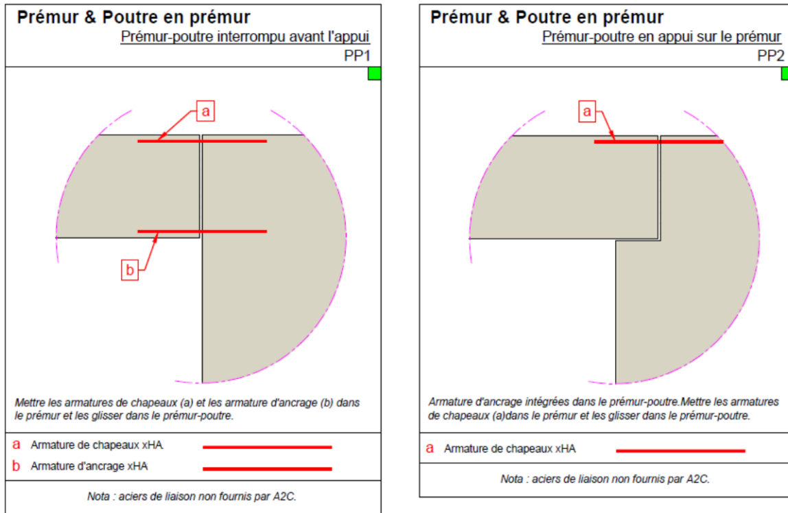
Figure 17 – POUTRES
