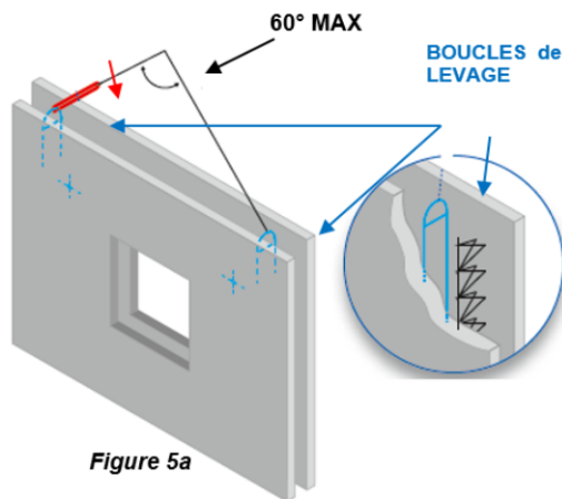
Figure 30 - Manutention des Prémurs A2C
