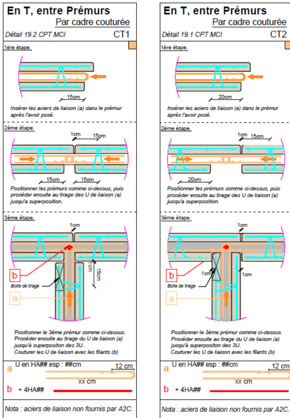
Figure 13 - LIAISONS COUTUREES - 2
